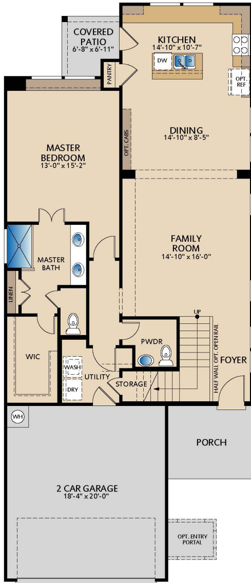
FIRST FLOOR
