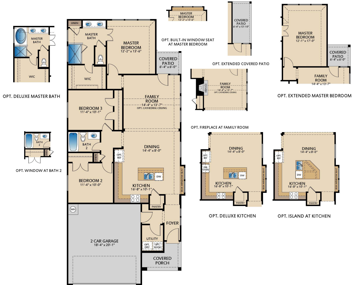
FLOOR PLAN
