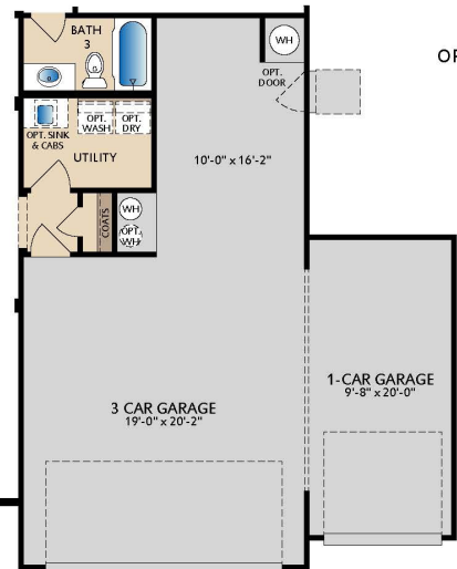
OPT. 4 CAR GARAGE
