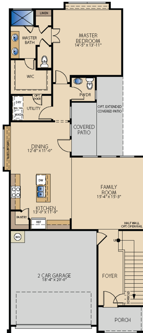
FIRST FLOOR
