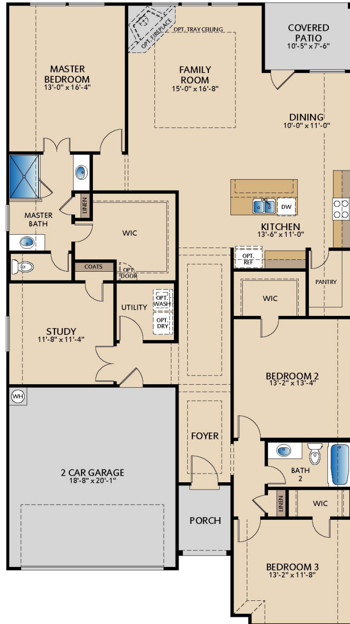
FLOOR PLAN
