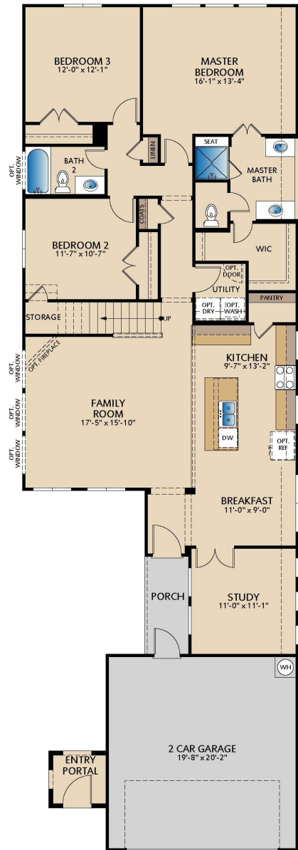
FIRST FLOOR W/ STAIRS TO OPT. SECOND FLOOR
