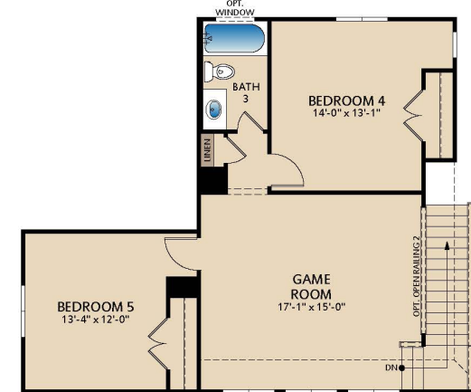
OPT. GAME ROOM, BEDROOM 4 & BEDROOM 5
