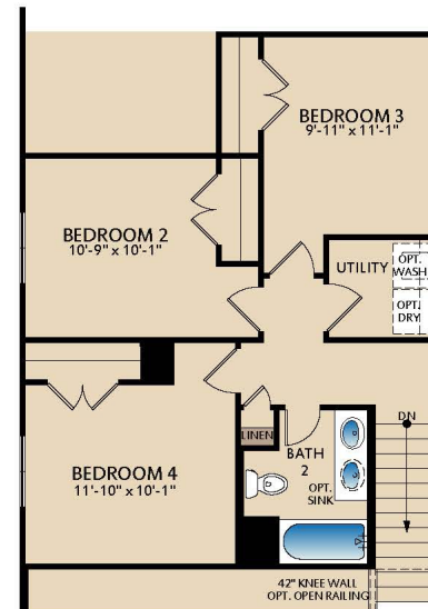
OPT. BEDROOM 4 AT LOFT
