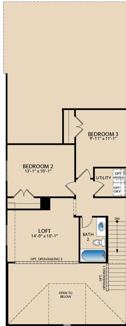
SECOND FLOOR
