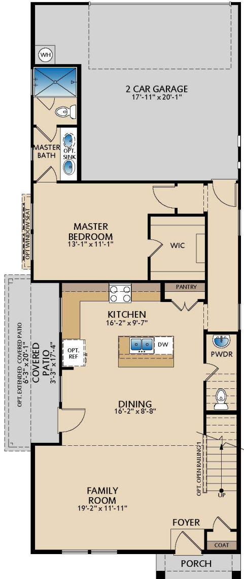
FIRST FLOOR
