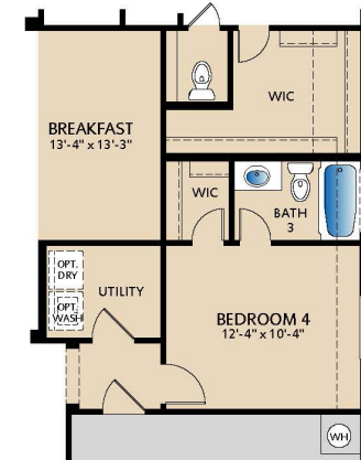
OPT. BEDROOM 4 W/ BATH 3 AT STUDY
