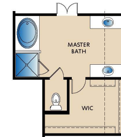
OPT. MASTER BATH W/ SECOND FLOOR
