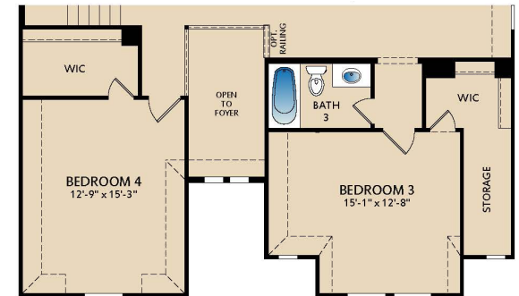
SECOND FLOOR ELEVATION D
