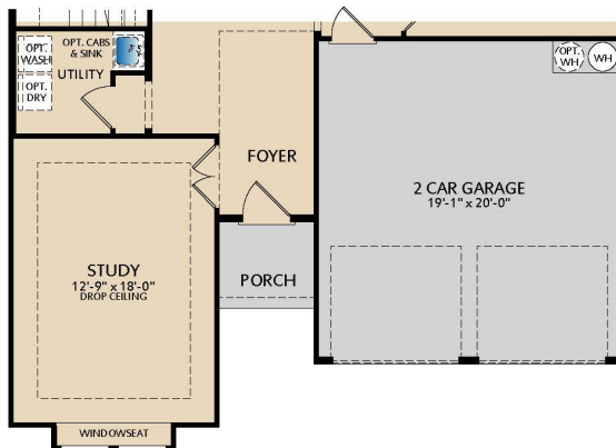
FIRST FLOOR ELEVATION D
