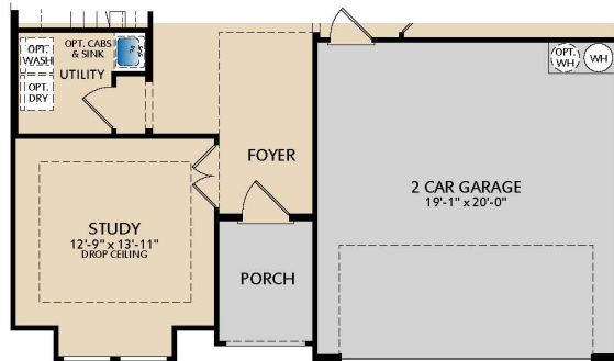
FIRST FLOOR ELEVATION B
