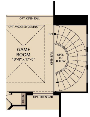
OPT. CIRCULAR STAIRS AT SECOND FLOOR
