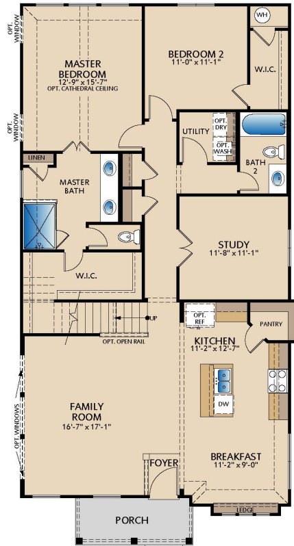
FIRST FLOOR 42264 R - MAJESTIC
