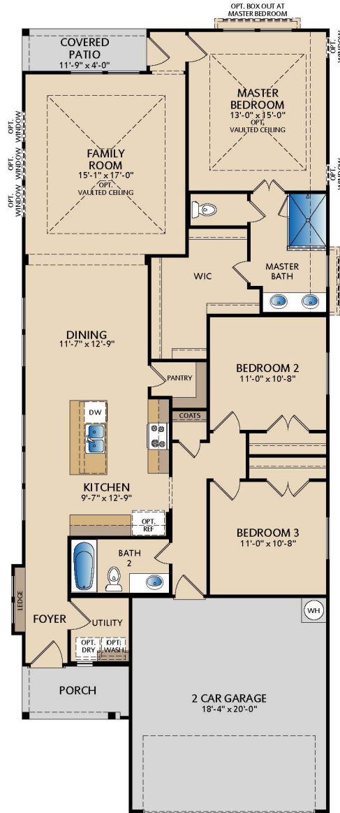
FLOOR PLAN
