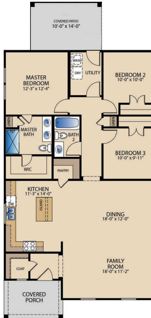
FLOOR PLAN
