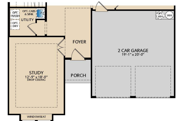
FIRST FLOOR ELEVATION D
